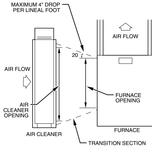
Fig. 4—Transition to Unit
