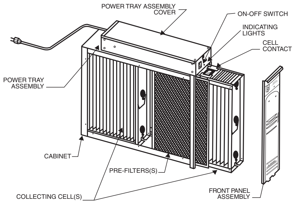
Fig. 1—EACB Electronic Air Cleaner
