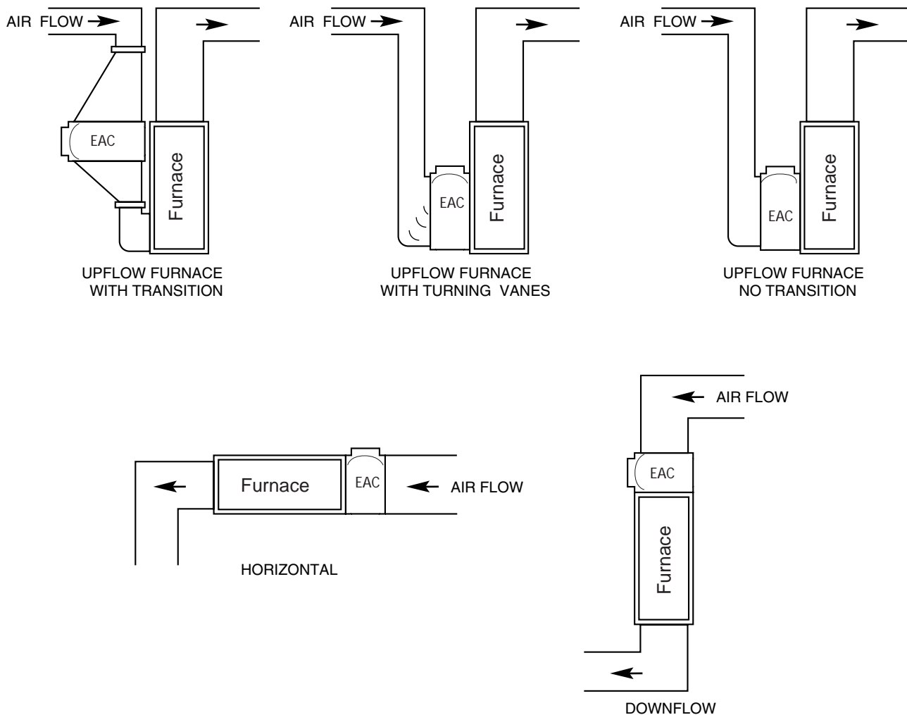
Fig. 7b—Typical Installations
