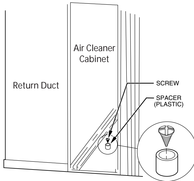
Fig. 6—Plastic Positioning Spacer
