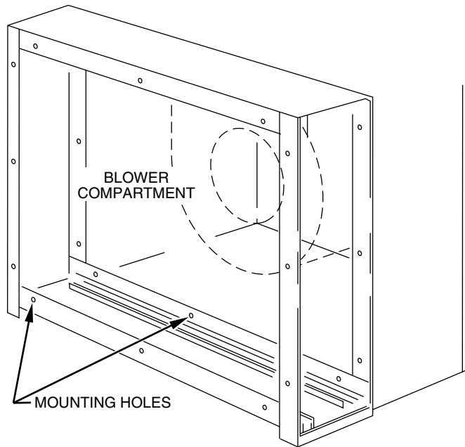
Fig. 8—Mounting Hole Location
